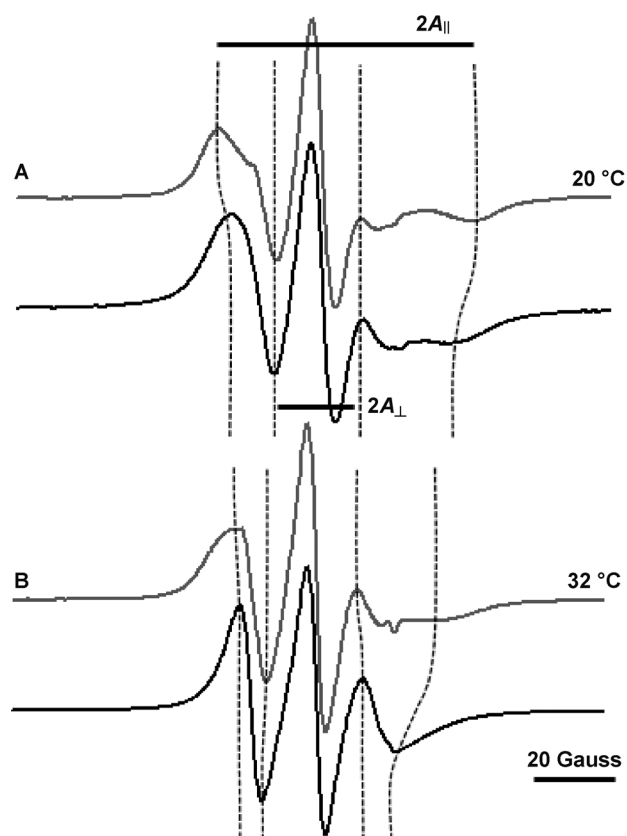
Figure 4. EPR spectra for 11-SASL incorporated into Lipodisq particles (upper spectra) and in a DMPC dispersion (lower spectra) at A) 20 °C and B) 32 °C. 2A_{\parallel} and 2A_{\perp} are indicated by dashed lines. [7] S_{app} can be calculated from S_{app} = (A_{\parallel} - A_{\perp}) / (A_{zz} - A_{xx}) , which is the ratio of the observed hyperfine anisotropy to the 25 Gauss maximum corresponding to rigid order, and defined by 0 > |S_{app}| > 1 where S_{app} = 1 is rigid and S_{app} = 0 is isotropically disordered. [8]
